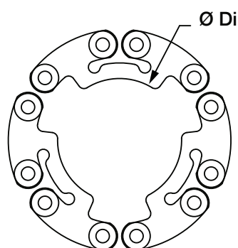
12-Bolt Disc-Pack
