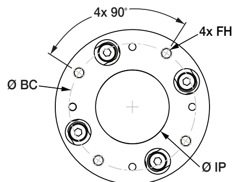
8-Bolt Flange
