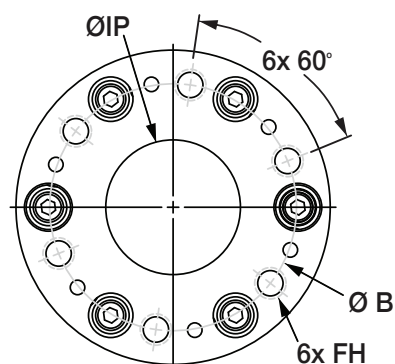
12-Bolt Flange
