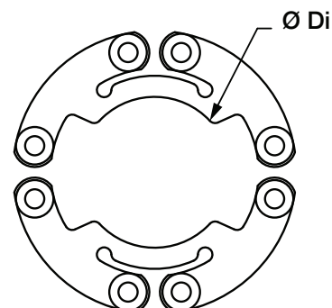
8-Bolt Disc-Pack
